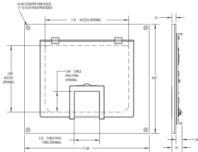
HATCH-500P-SLD5
