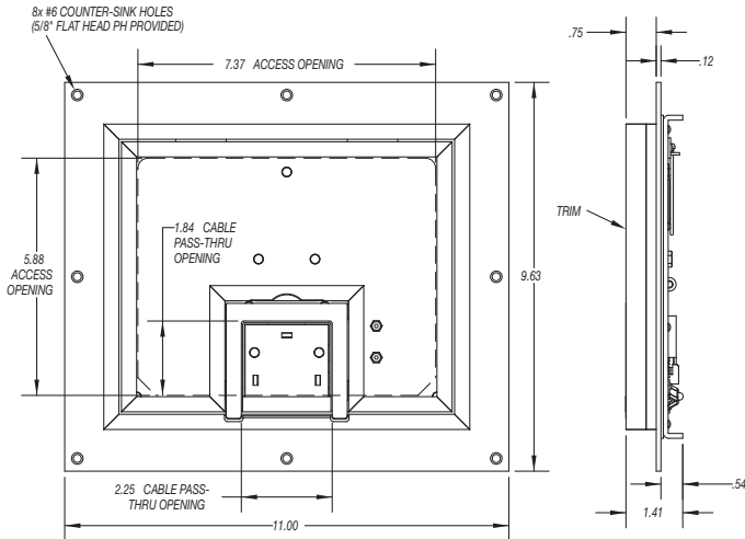
HATCH-500P-X75
