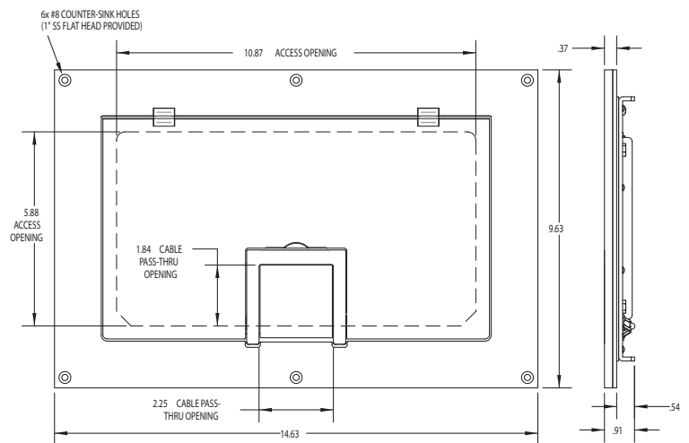
HATCH-600P-SLD
