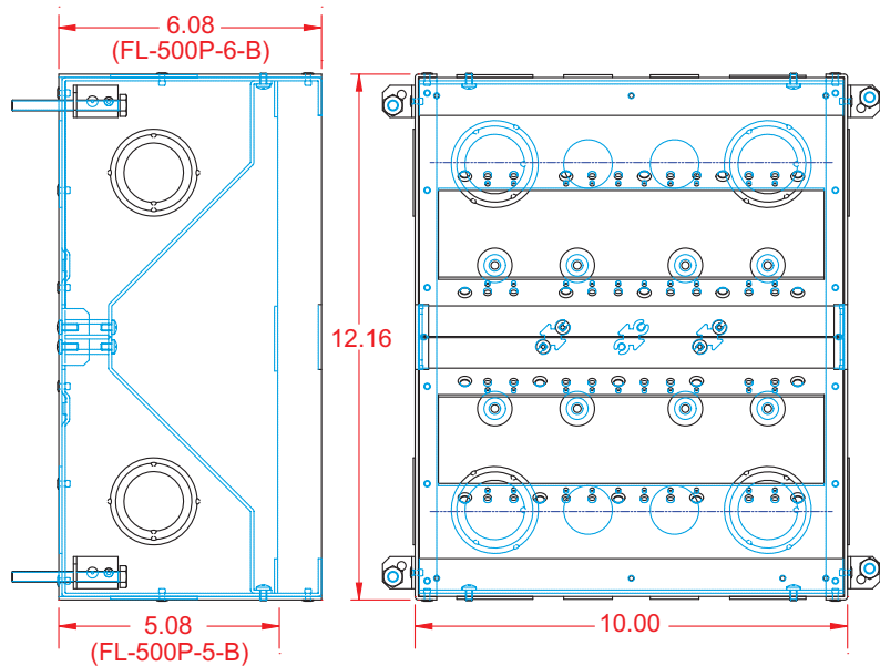
FL-500P-5-B & 6-B 5" & 6" Deep
