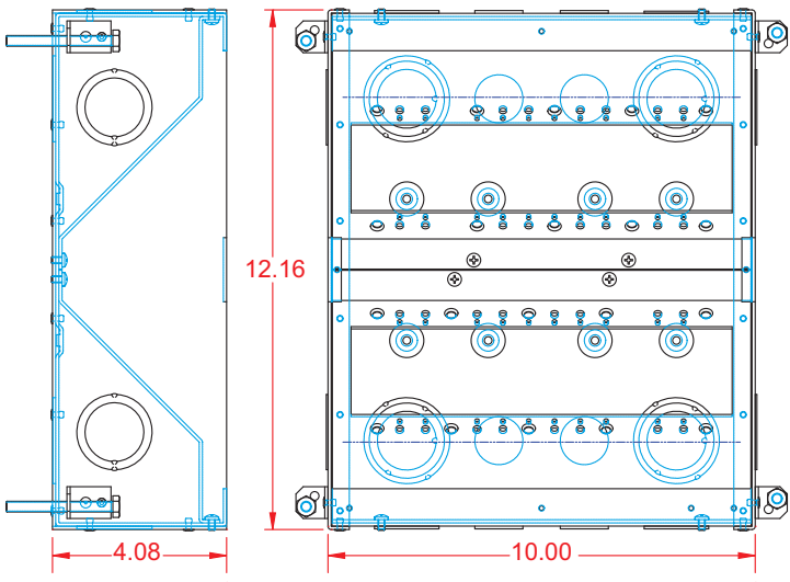
FL-500P-5-B & 6-B 5" & 6" Deep
