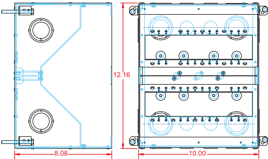
FL-500P-8-B 8" Deep
