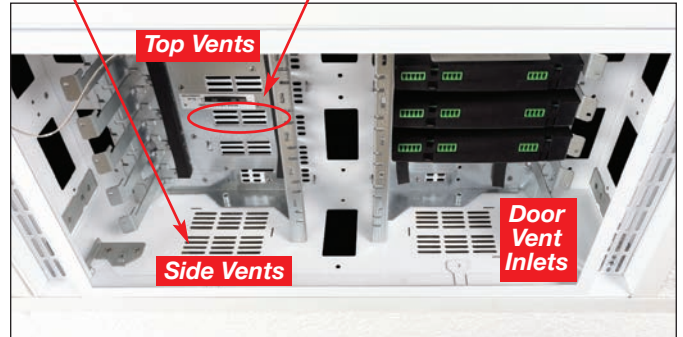
CB-12-PTF Vent Locations
