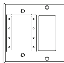
IPS-WP2D 2 Gang Plate w/1 IPS & 1 Decora (see IPS and SS Series Spec Sheet)
