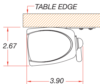
"CA" OR "CC" INSERT ("CC" SHOWN)
