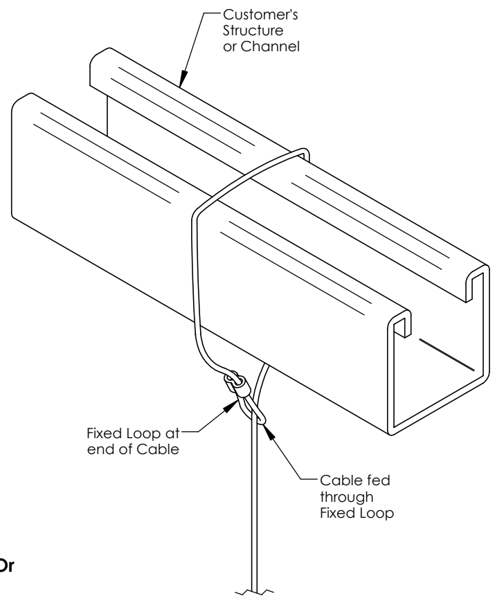
Cable with Fixed Loop
