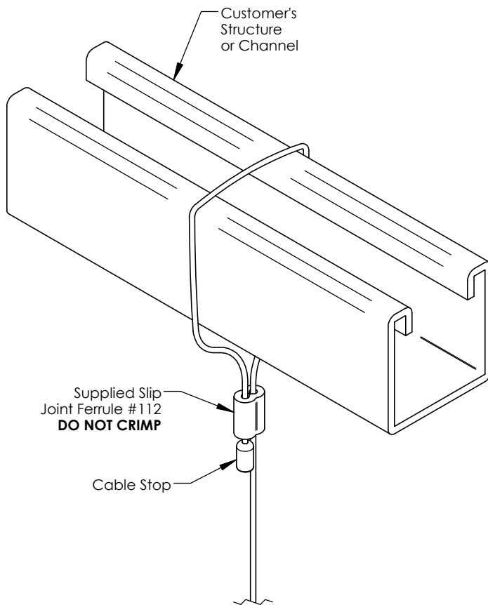
Cable with Stop and Ferrule
