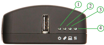
USB-EXT-1 Remote Extender shown
