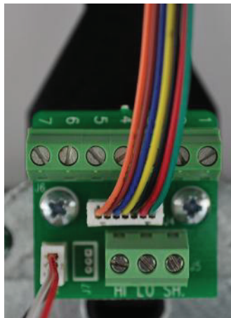
Plug the wire harness to this header as shown.
