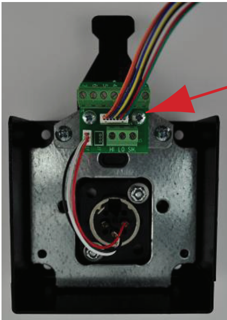
Plug the wire harness to this header as shown.
