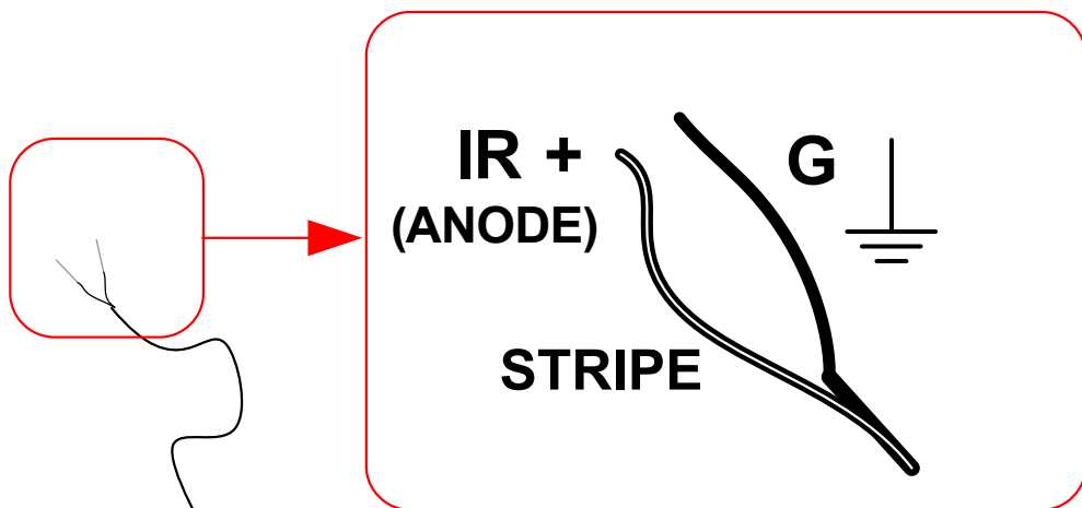
FSR IR EMITTER CABLE 28397 PINOUT
