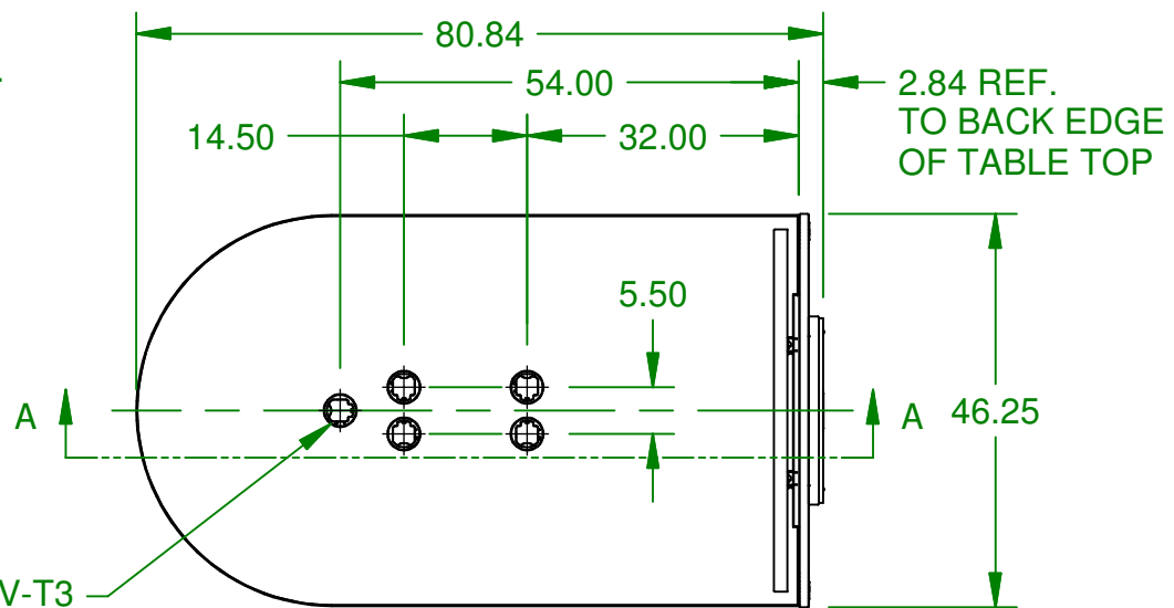
LAYOUT D SCALE 0.04 : 1
