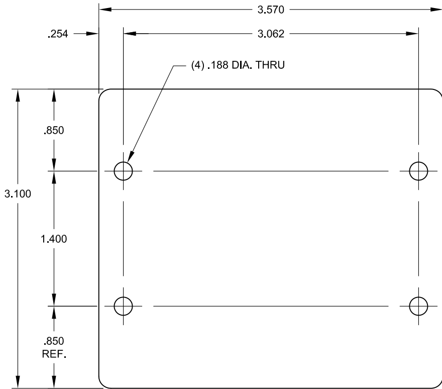
BLANK PLATE FOR FL-5x0P4"-CRST-DMtx P/N 99509
