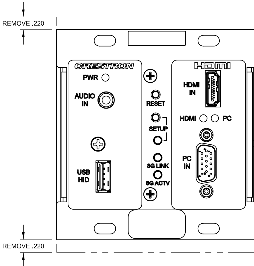
CRESTRON DM-Tx-200C-2G MODIFICATION REMOVE INDICATED AREA OF FACE PLATE SO THAT UNIT WILL FIT INSIDE FLOOR BOX
