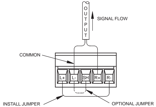
TO A MONO BALANCED PREAMP INPUT
