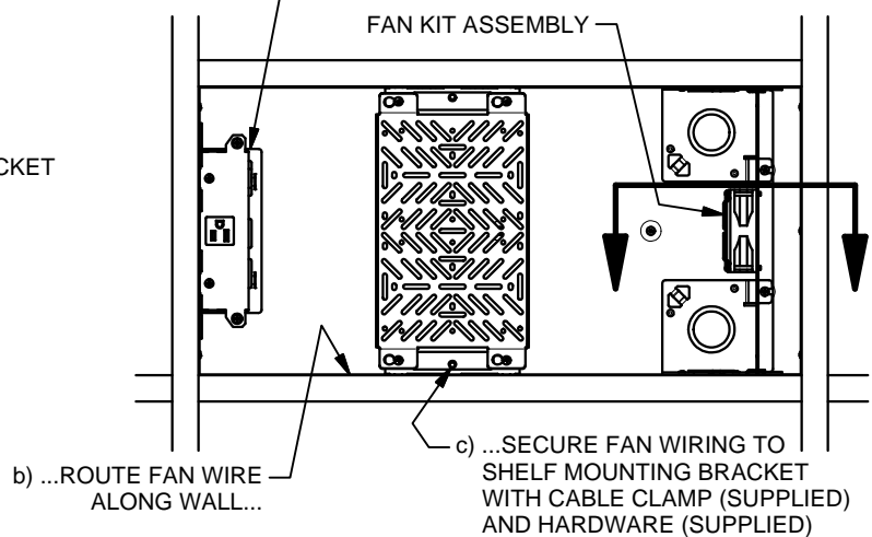
BOTTOM VIEW SHOWING FAN KIT ASSEMBLY INSTALLED
