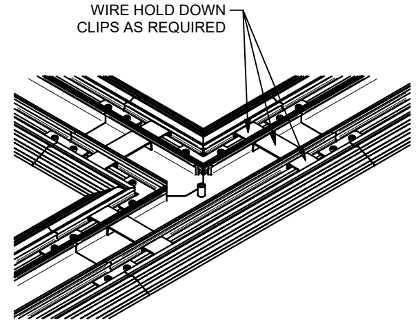
ASSEMBLED VIEW WITH RACEWAY BASE SECTIONS
