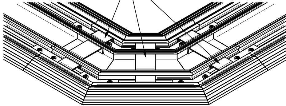
ASSEMBLED VIEW WITH RACEWAY BASE SECTIONS
