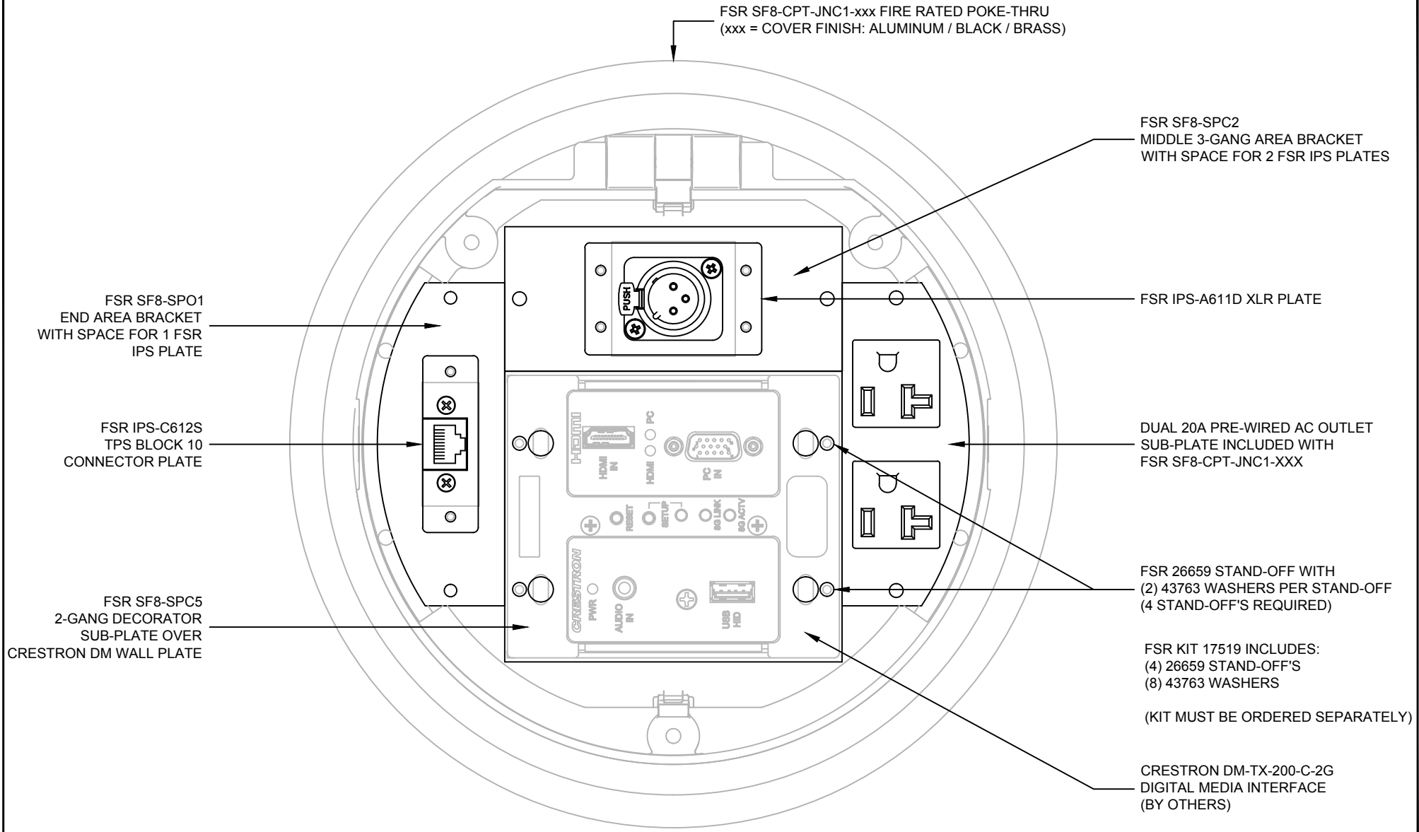
1 FSR SF8-CPT-JNC1-xxx FIRE RATED POKE-THRU TOP VIEW (INTERNAL)
