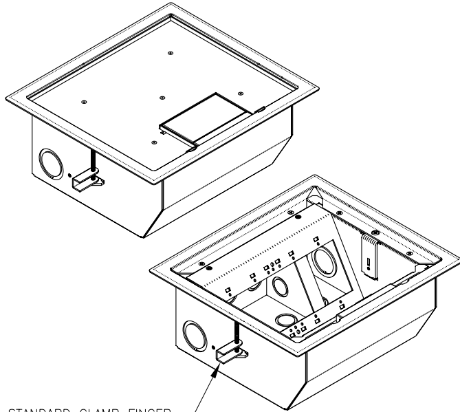
STANDARD CLAMP FINGER
