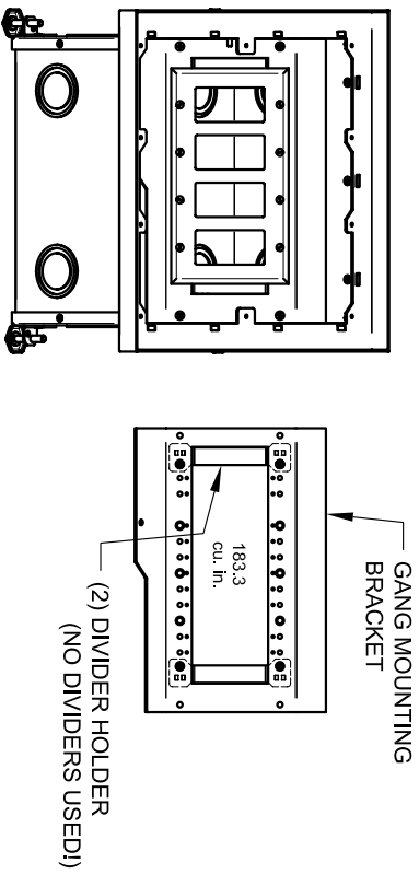
4-GANG CONFIGURATION
