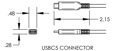
USBC5 CONNECTOR
