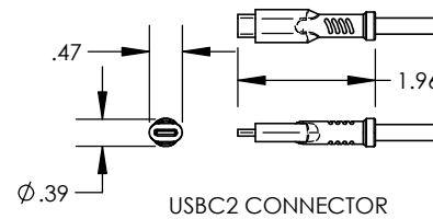
USBC2 CONNECTOR
