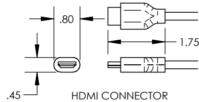
HDMI CONNECTOR
