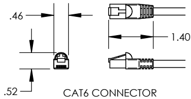
CAT6 CONNECTOR
