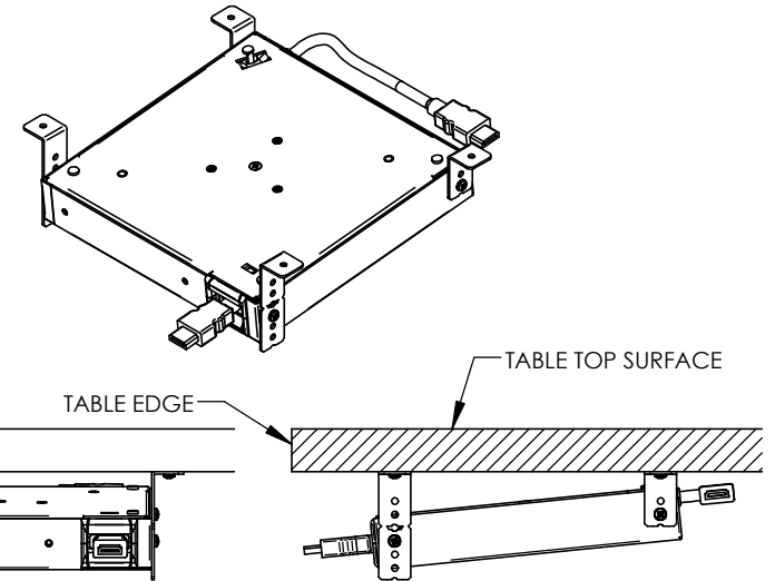
ANGLED CPRT MOUNTING (CAN MOUNT UP TO 2 CPRT RETRACTORS)
