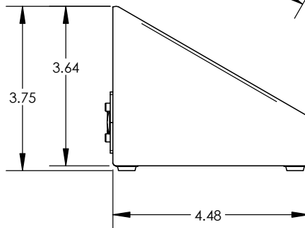
END VIEW
