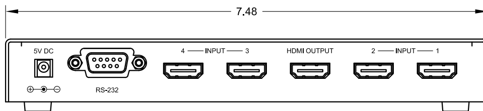
BACK VIEW
