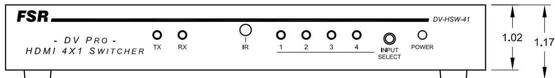
FRONT VIEW
