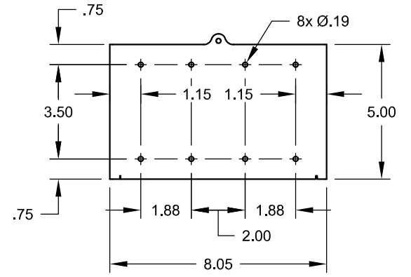
WALL MOUNT MOUNTING PLATE
